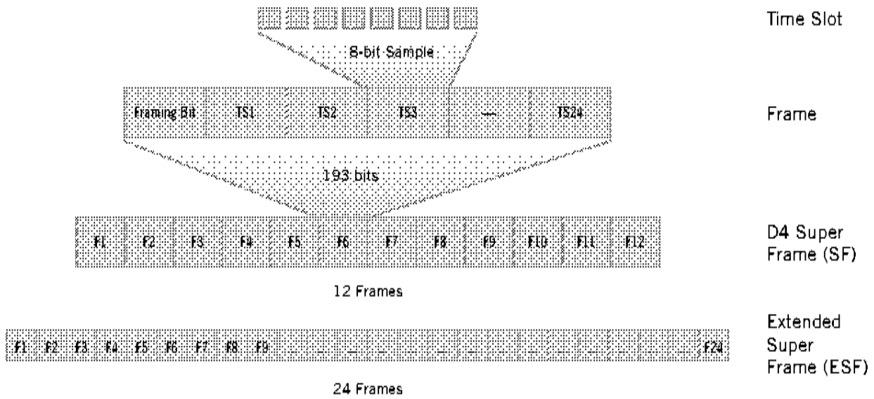
Figure 2. Robbed Bit Framing
